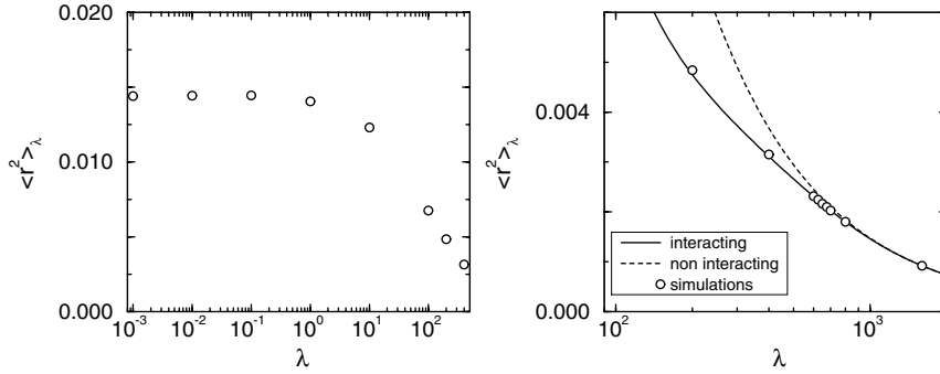
Figure 10.3: The mean-squared displacement \langle r^2 \rangle_\lambda as a function of the coupling parameter \lambda for a hard-sphere (fcc) solid of 54 particles (6 layers of 3 \times 3 close-packed atoms at a density \rho = 1.04 ). The figure on the left shows the simulation results for low values of \lambda , the figure on the right for high values. The solid line takes into account nearest-neighbor interactions (10.3.31); the dashed line assumes a noninteracting Einstein crystal (10.3.30). The open symbols are the simulation results.
