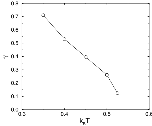
Figure 17.2: Surface tension as a function of temperature.
