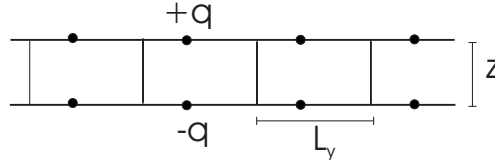
Figure 12.6: A system containing two point charges at positions (\mathbb{Q}, \quad) and (\mathbb{Q}, \quad) ; because of the periodic boundary conditions in the x and y directions, two oppositely charge “sheets” are formed. There are no periodic boundary conditions in the z direction.
