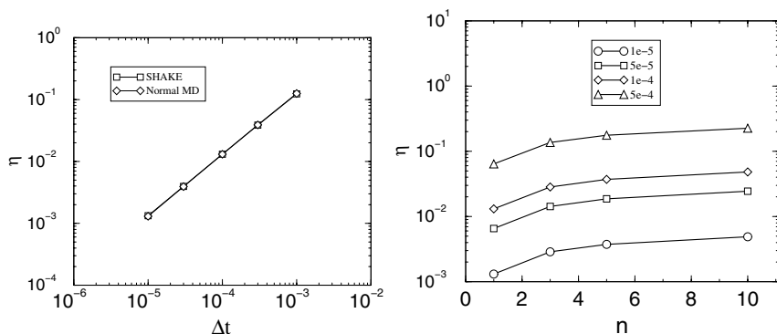
Figure 15.3: Comparison of the efficiency \eta for bond constraints (SHAKE) with normal molecular dynamics (left), and multiple times steps (right). The left figure gives the efficiency as a function of the time step and the right figure as a function of the number of small time steps n , \Delta t = n\delta t , where the value of \delta t is given in the symbol legend.
