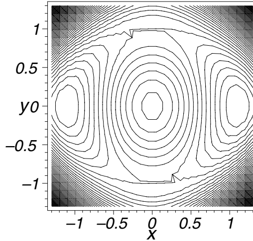
Figure 16.5: Contour plot of the function V(\mathbf{x}) defined by equation (16.4.20). The two minima are at (-1, 0) , A, and (1, 0) , B. These minima are separated by a potential energy barrier.
